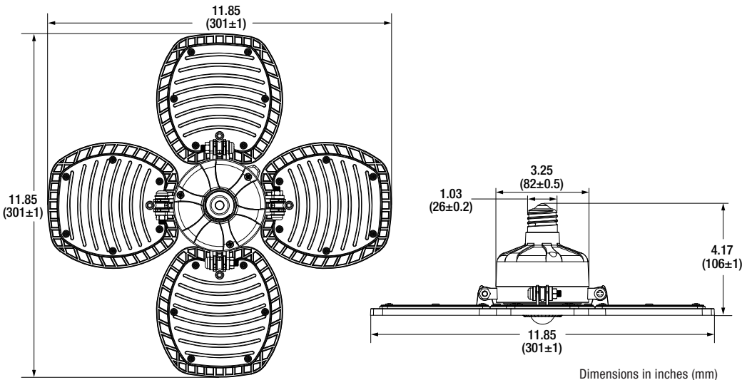
Dimensions in inches (mm)
